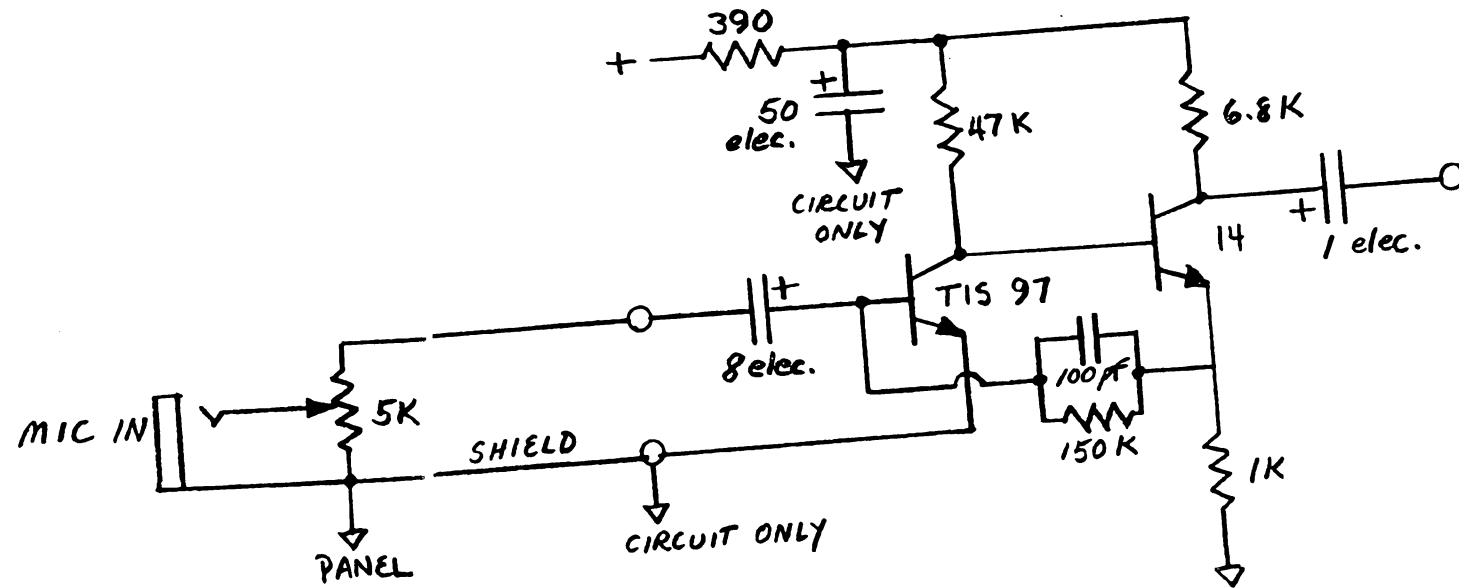
MIC PREAMP
